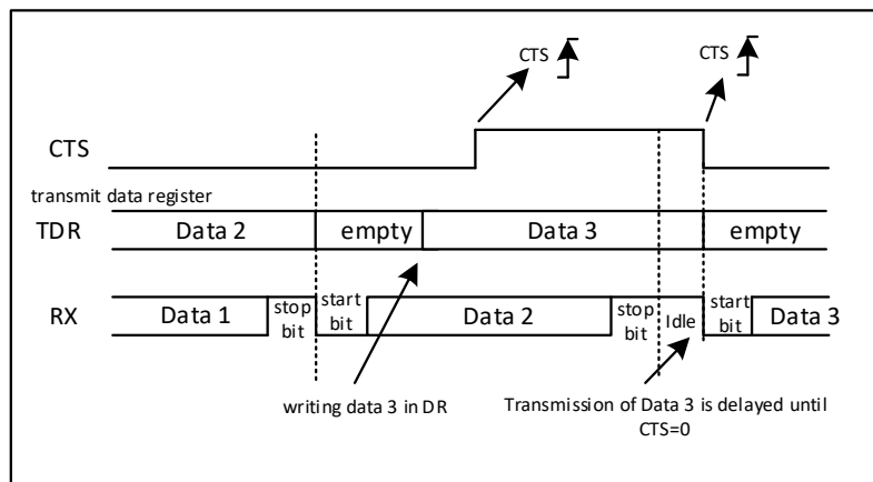
Figure 20-15 CTSflow control
