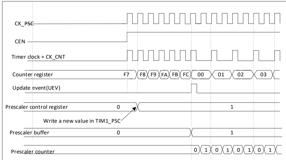
Figure 16-1 Counter timing diagram with prescaler division change from 1 to 2
