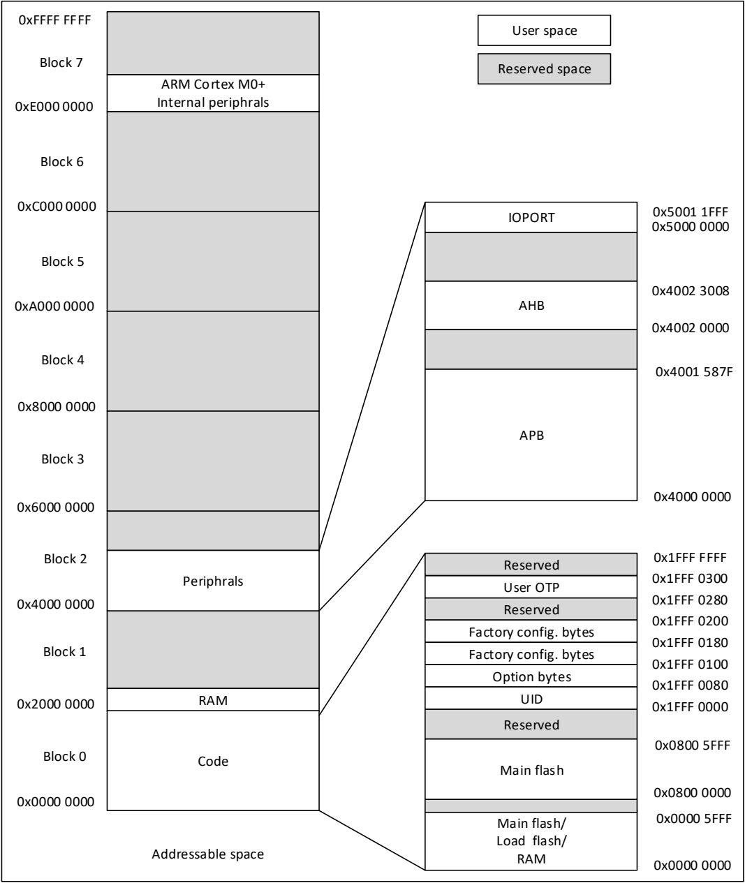
Figure 3-2 Memory map
