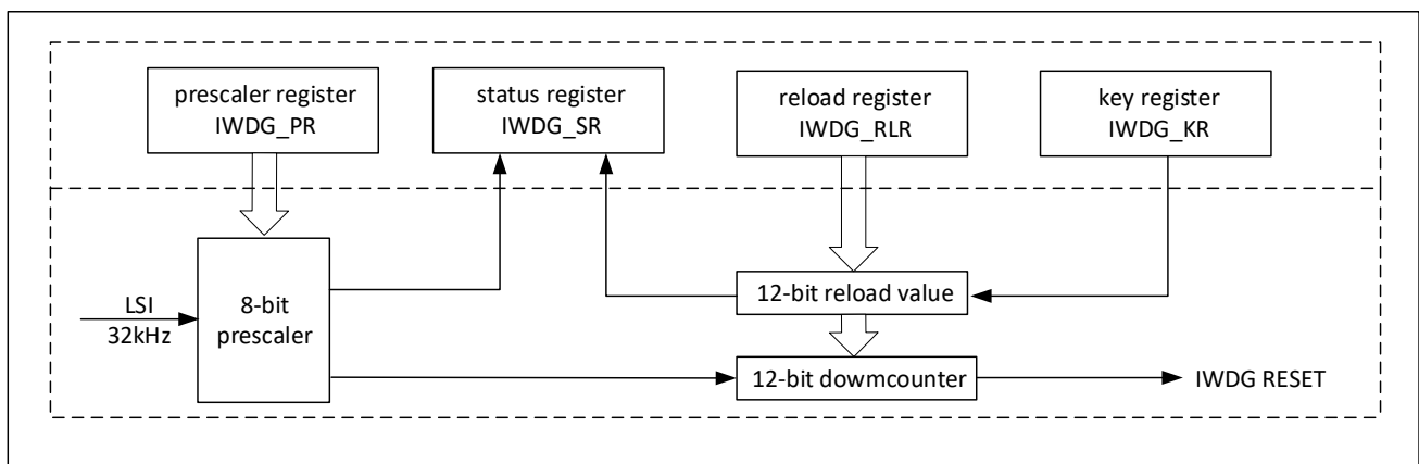
Figure 18-1 IWDGblock diagram
