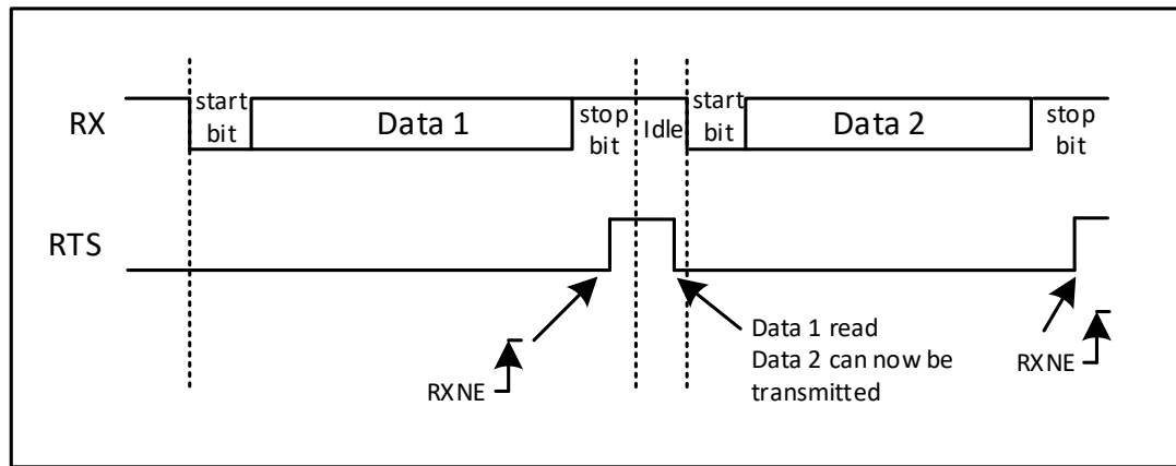
Figure 20-14 RTSflow control
